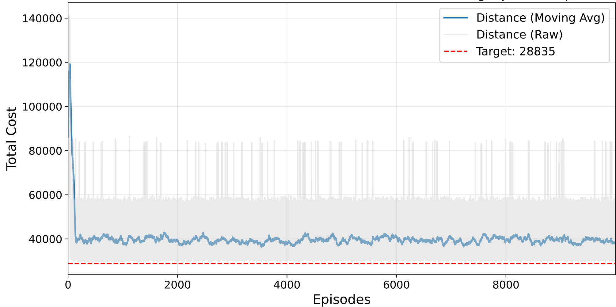
Final HYPERBAND TPE Masked AutoRL-SOP Training - p43.3.sop
